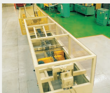
靜水壓重複彎曲試驗 Flexural Test for Hydrostatic Pressure
