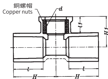
龍T入銅接頭 Faucet Fitting—Fixture TEE
