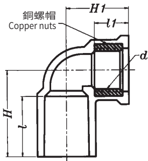
龍入銅接頭 Faucet Fitting—90° Elbow
