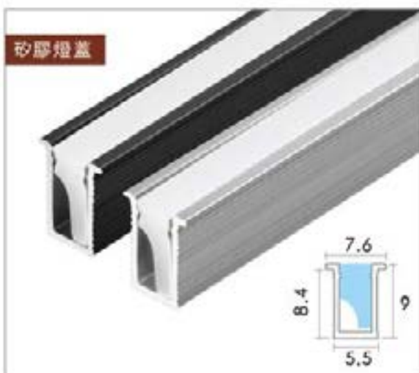
LAD1082 矽膠嵌入硬條燈
