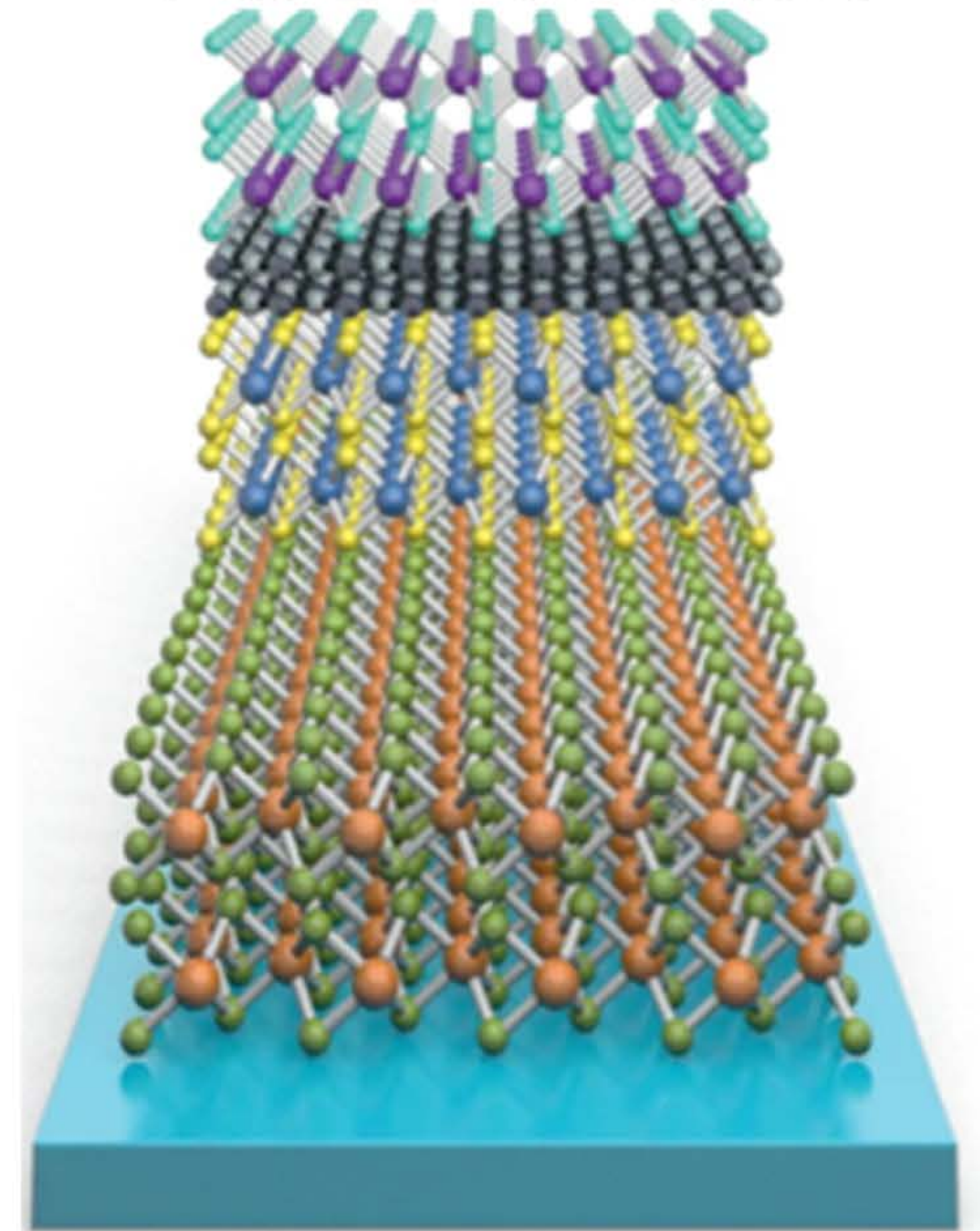
All 2D-MRAM
