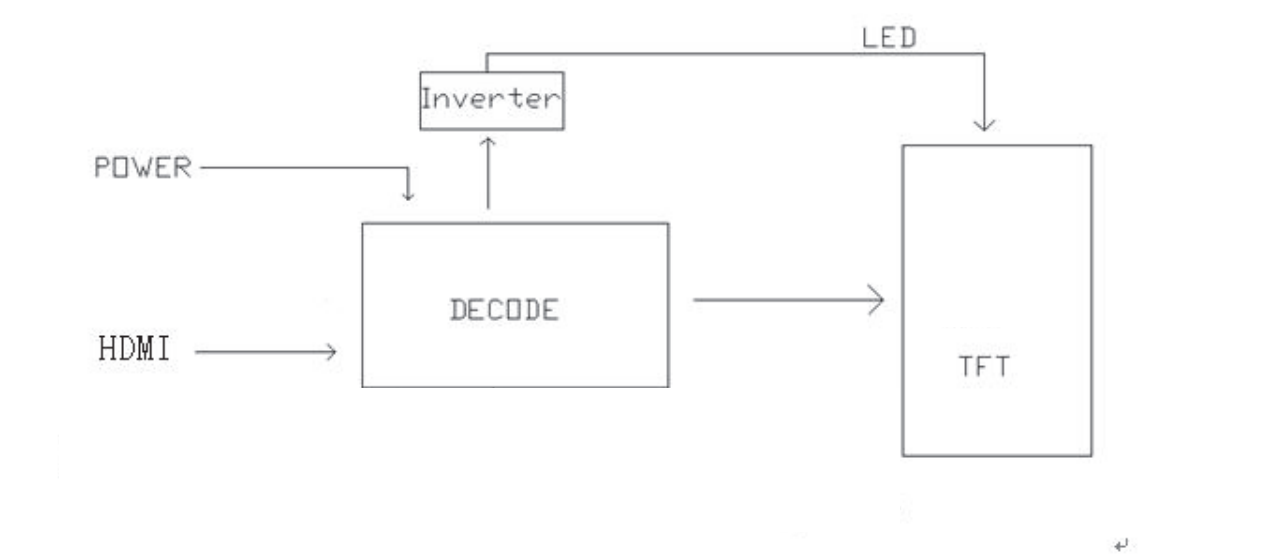
Block Dimension
