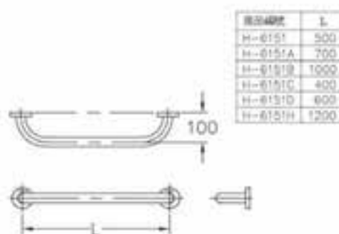
H-6151C 400長×100寬mm $2,800 H-6151 500長×100寬mm $2,900 H-6151D 600長×100寬mm $3,100 H-6151A 700長×100寬mm $3,200 H-6151B 1000長×100寬mm $3,800 H-6151H 1200長×100寬mm $4,100 C型扶手 1½" f 註：附膨脹螺絲6支 材質：不銹鋼#304 (管徑 f 31.8mm)
