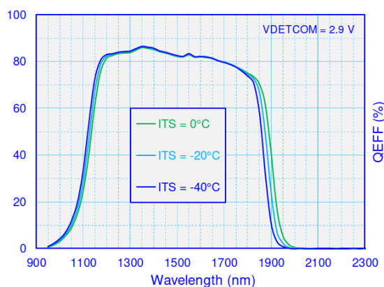
QE Spectrum
