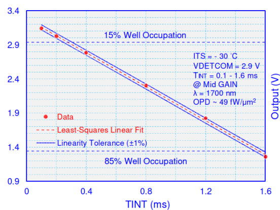
Output Linearity
